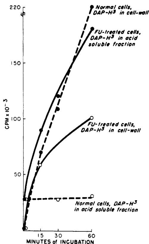
FIG. 5.—Incorporation of H^3 -DAP into E. coli K-12 in the presence (100 \mu g/ml ) and in the absence of 5-fluorouracil. Experimental details are given in the text. Owing to technical difficulties no 0 minute sample was taken; the earliest sample represents 3rd minute of incubation.
